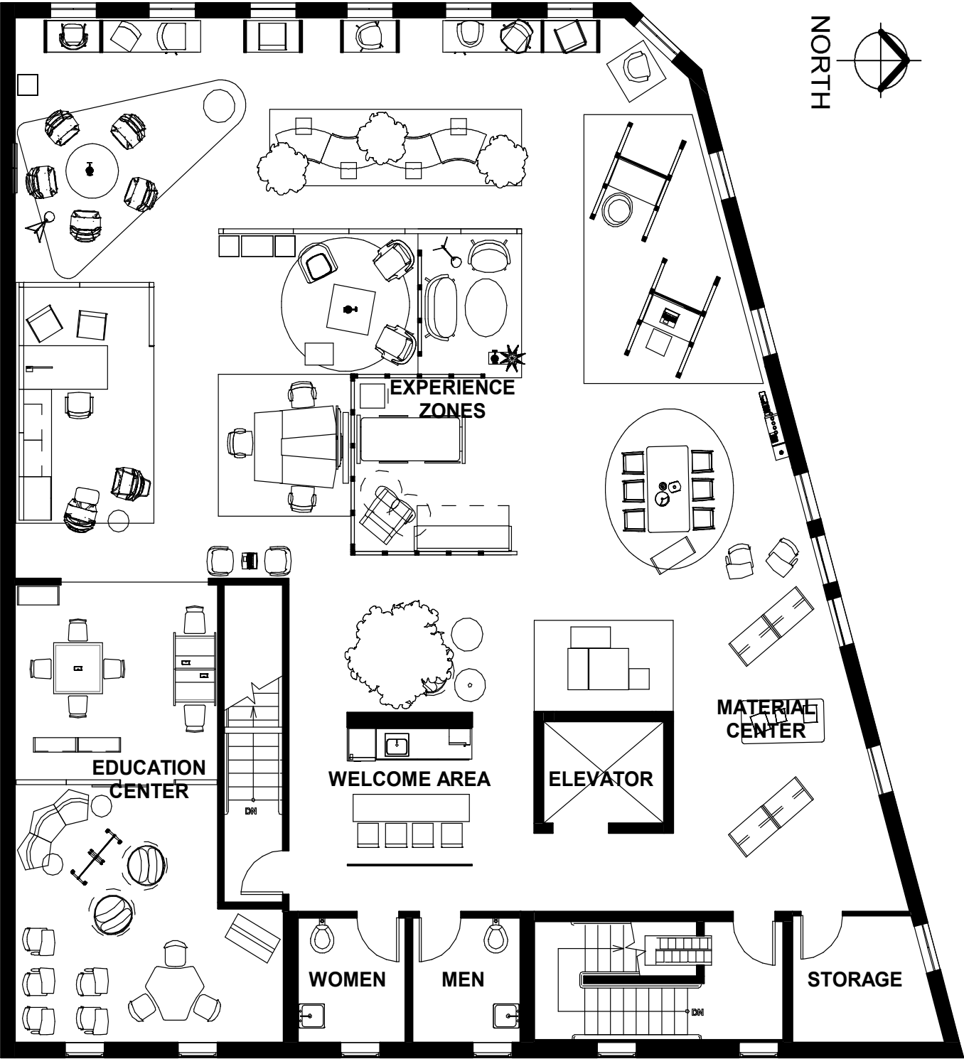
FLOOR PLAN
