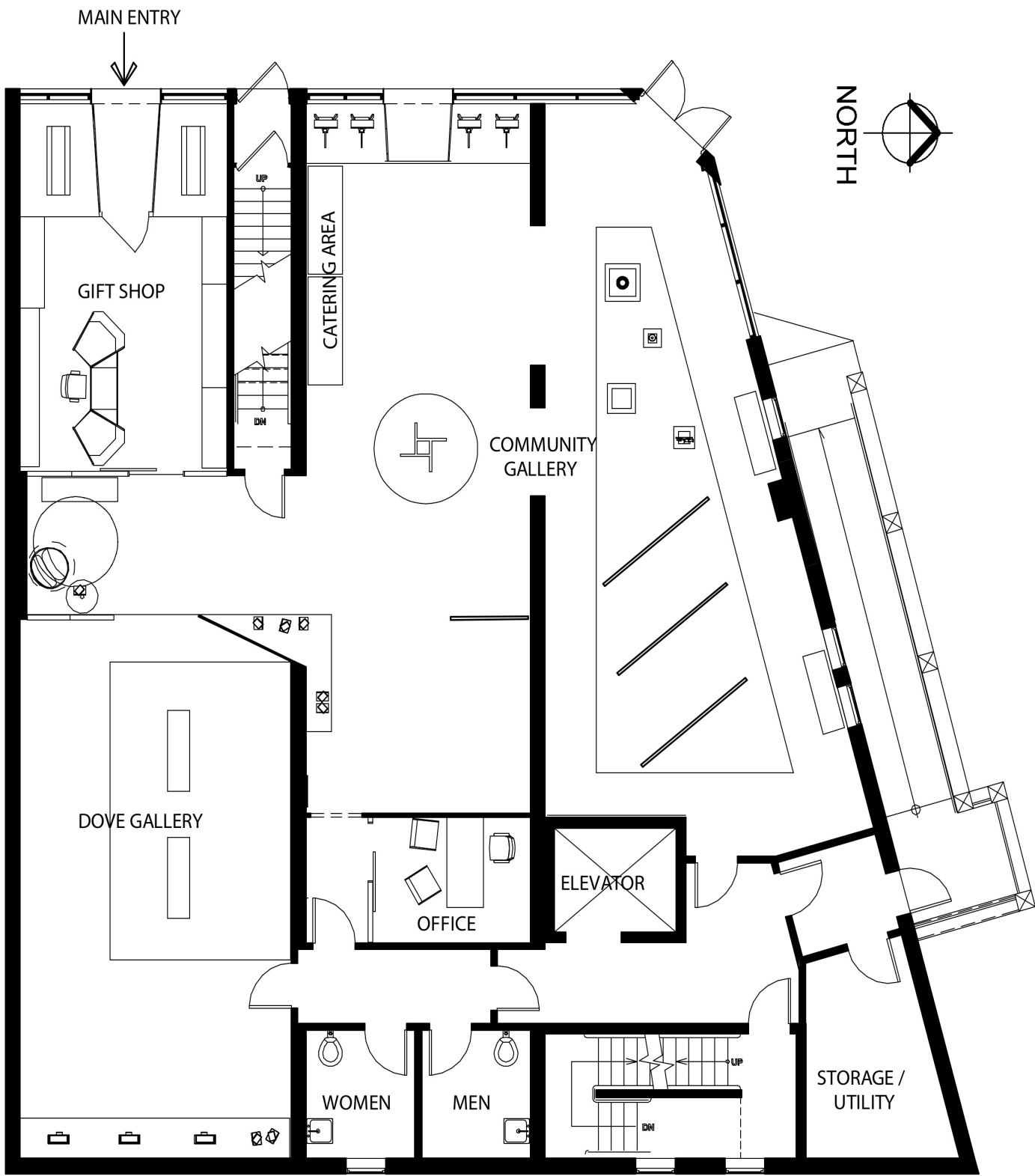
FLOOR PLAN
