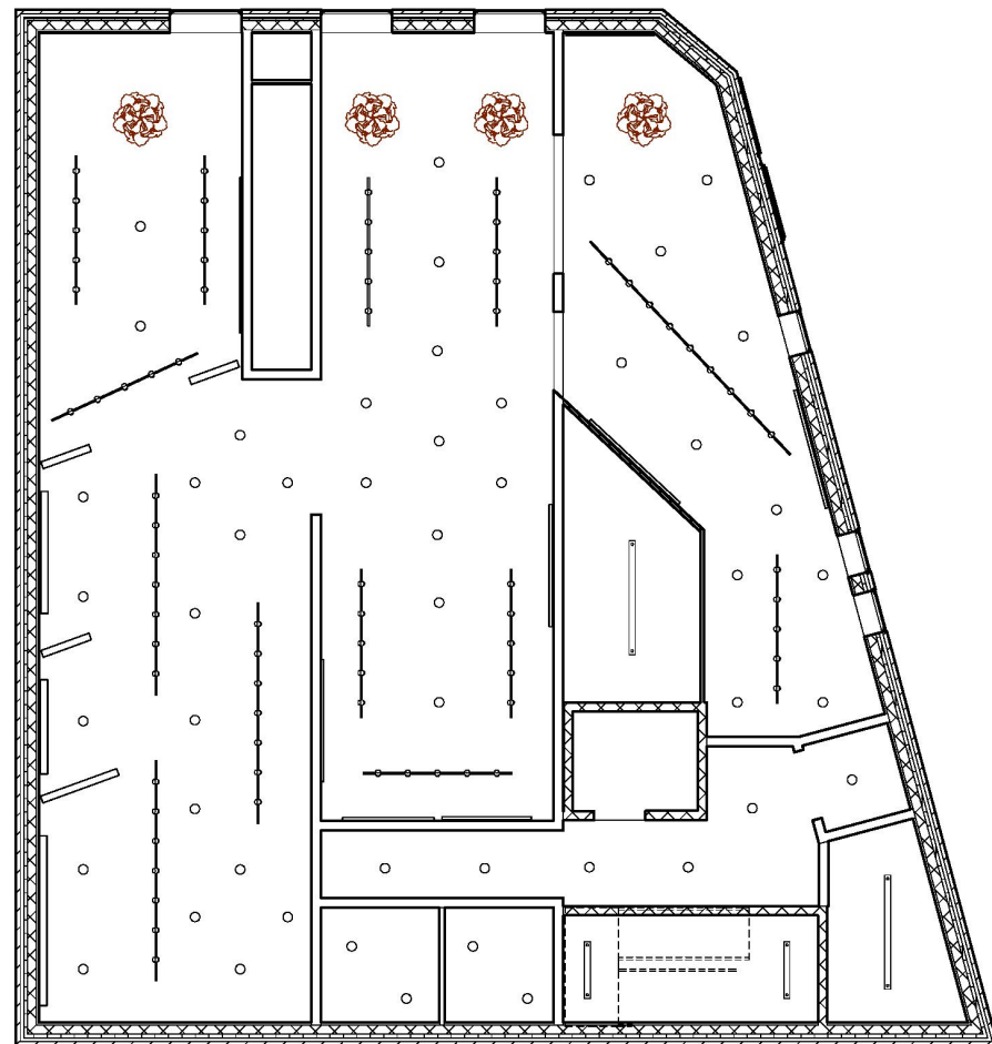
Level 1 Reflected Ceiling Plan
