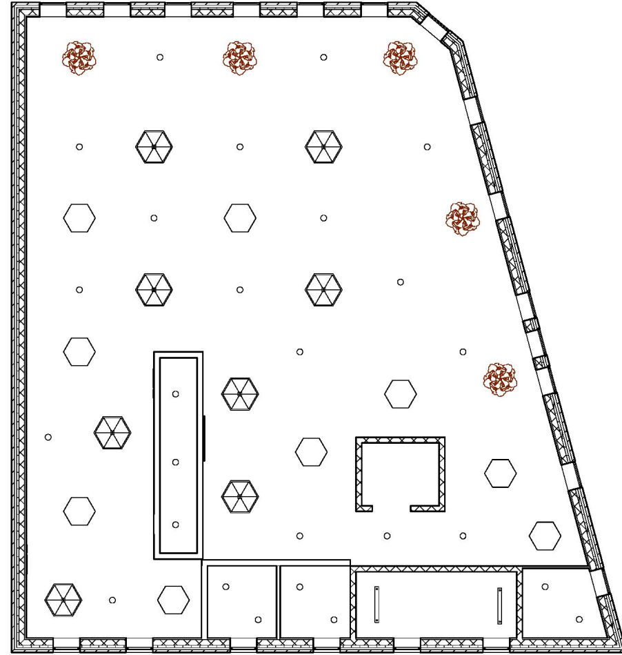
Level 3 Reflected Ceiling Plan
